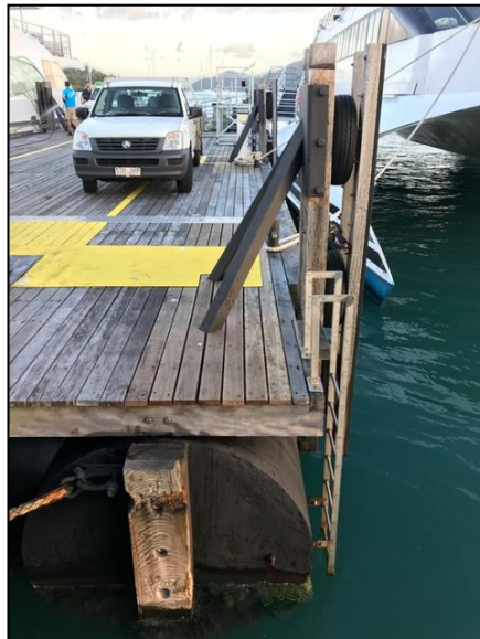
After shot of fenders and before shot of pontoon tube
