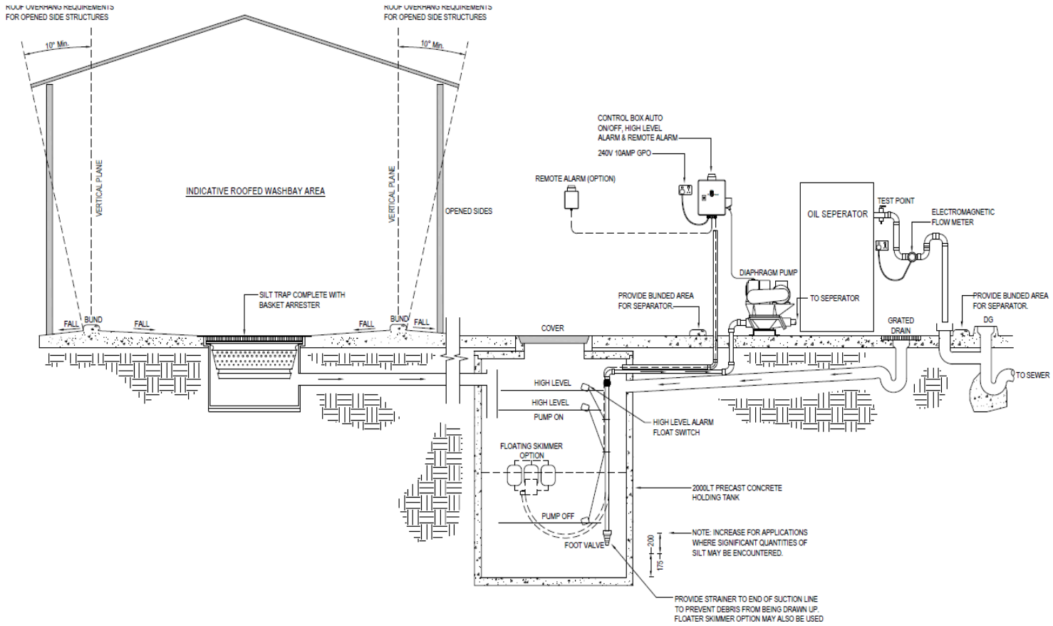
INDICATIVE ROOFED VEHICLE WASH BAY, HOLDING TANK AND OILS SEPARATOR DETAIL
