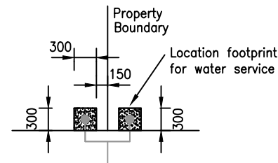
TYPICAL SERVICE INSTALLATION SETUP
