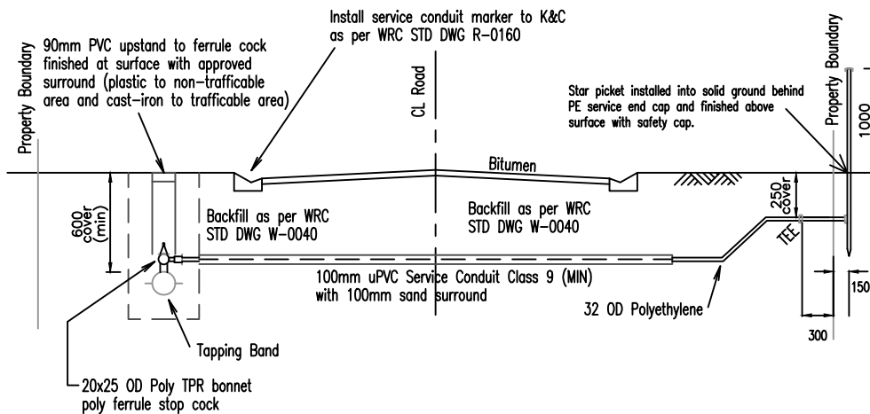
TYPICAL SECTION
