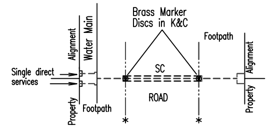
SERVICES LAYOUT
