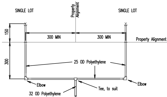
20mm MULTIPLE SERVICES DETAIL AT PROPERTY LINE
