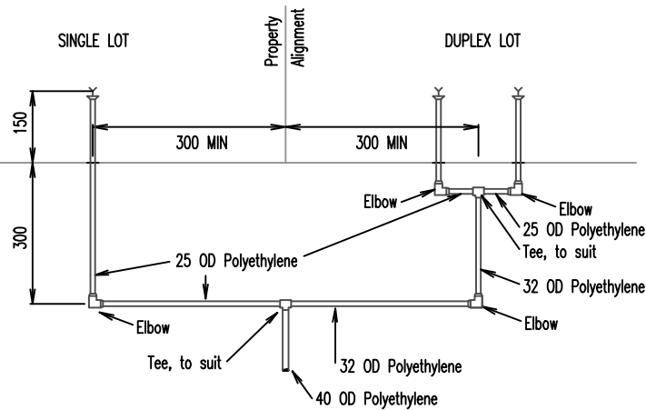
25mm DUPLEX & MULTIPLE SERVICES DETAIL AT PROPERTY LINE (ALTERNATIVE 1)
